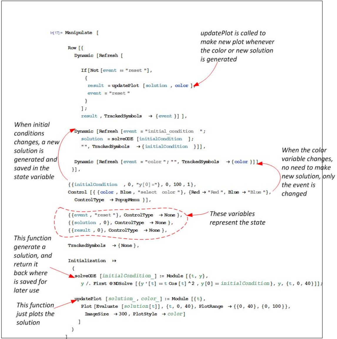
Figure 5: Manipulate code
