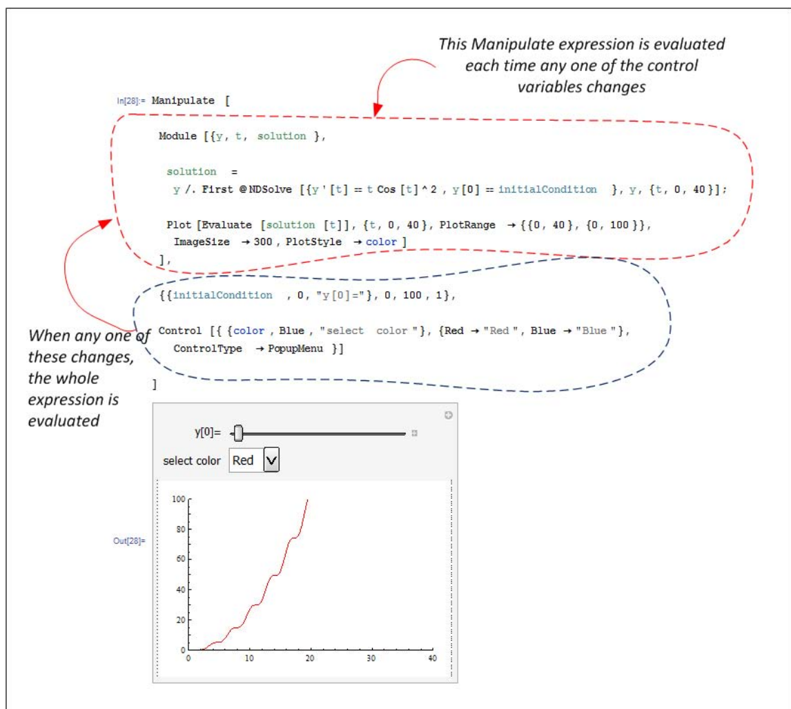
Figure 6: Manipulate code
