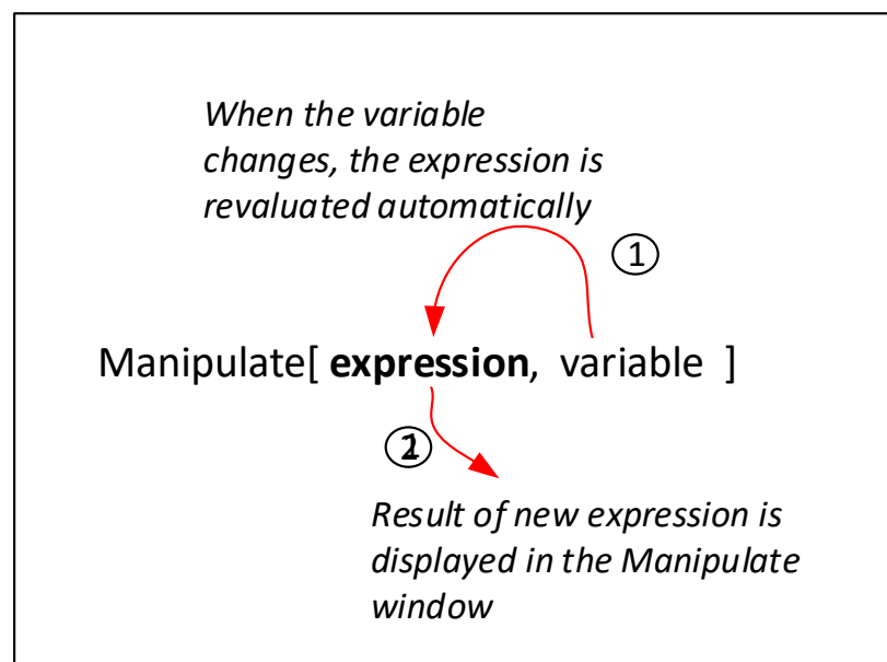
Figure 1: Manipulate logic
