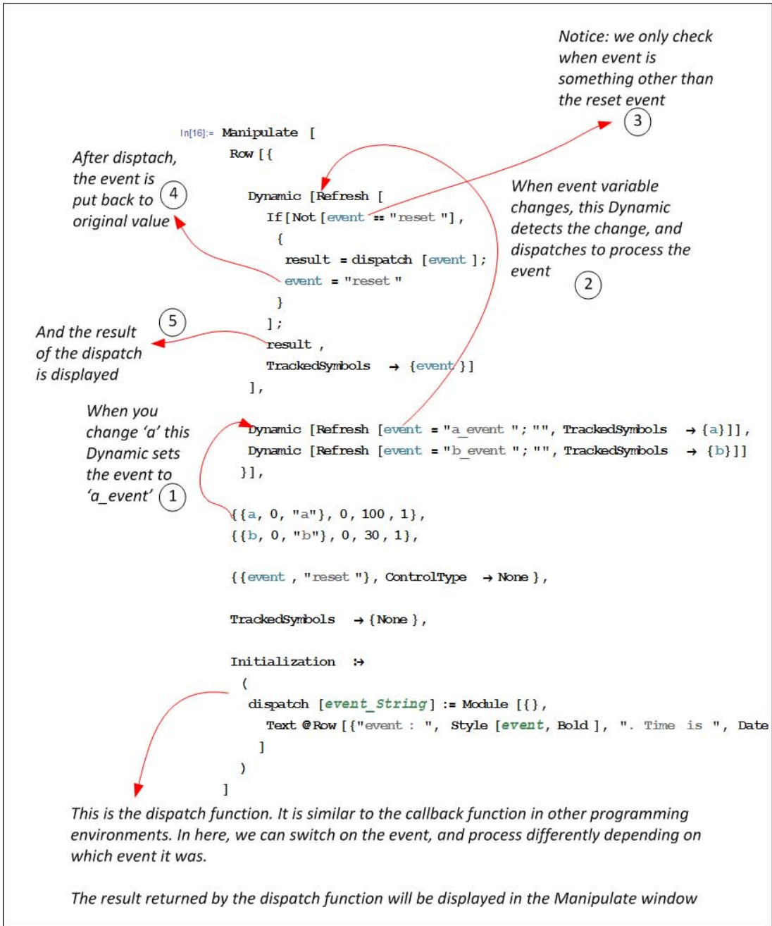
Figure 3: Manipulate code
