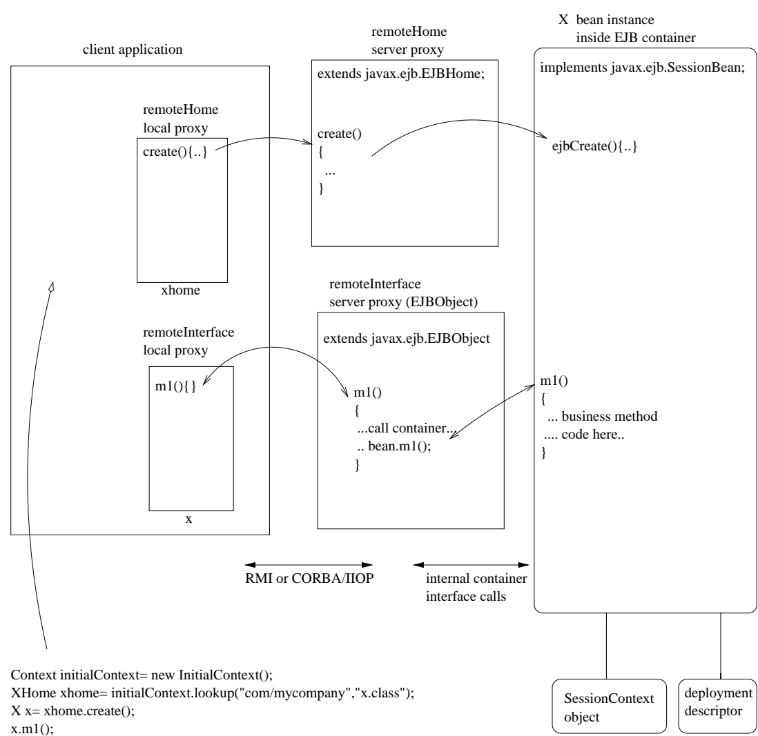
Figure 4: Container, Home, Remote, and bean relationship. view2.fig
