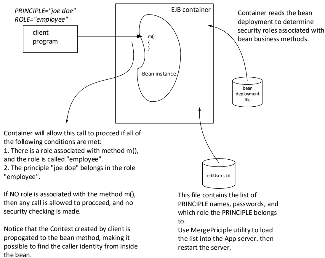
Figure 1: Overview of EJB security concepts. ejb_sec_1.vsd
