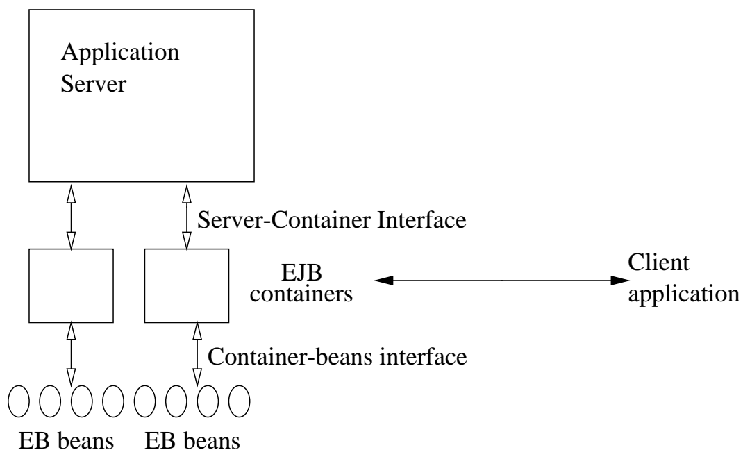
Figure 3: Server, Container and EJB instances. view1.fig
