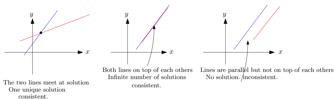
Figure 2: Possibilities for nonhomogeneous system
