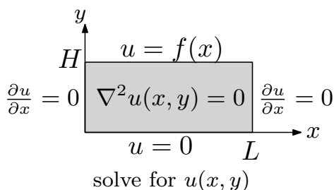
Figure 4.6: PDE specification
