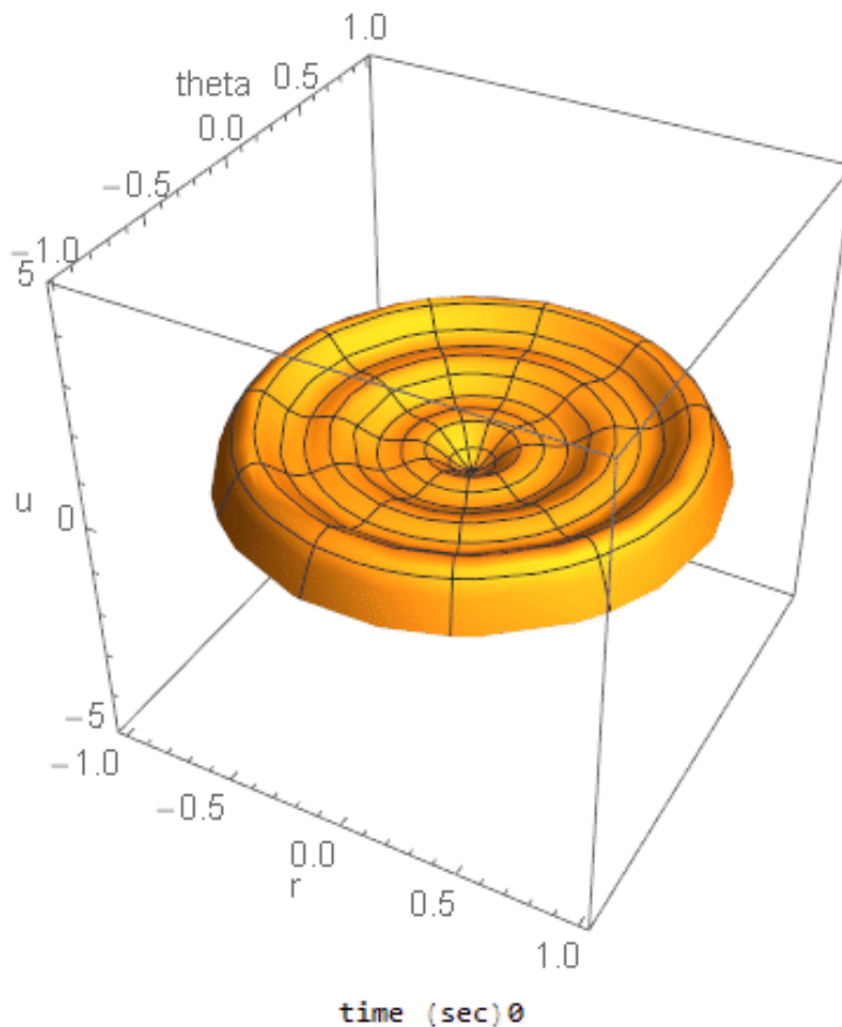
Figure 5.124: snap shot
