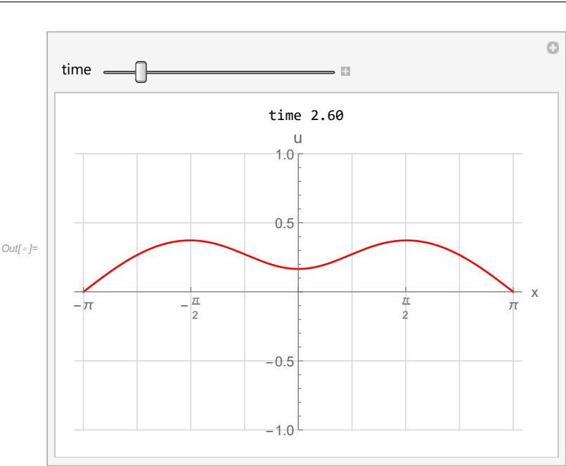
Figure 5.11: snap shot
