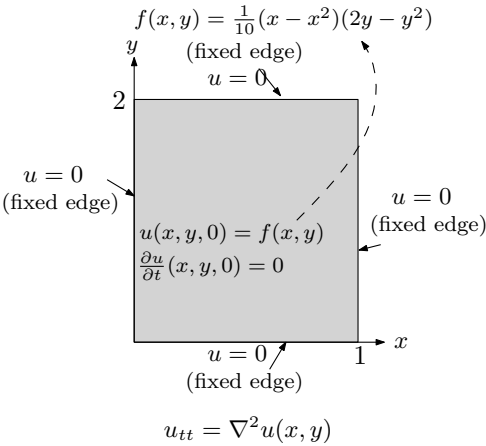
Figure 5.115: PDE specification
