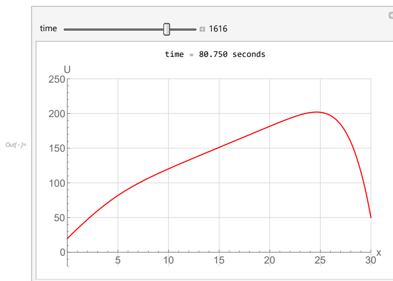
Figure 3.105: Initial state
