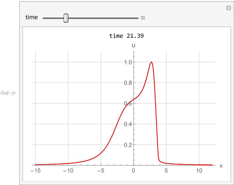
Figure 2.15: snap shot
