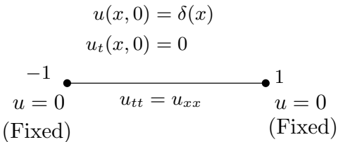
Figure 5.13: PDE specification
