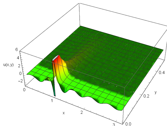
Figure 4.4: Plot of u(x, y)
