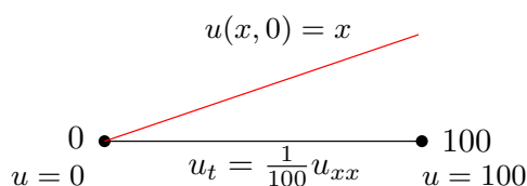
Figure 3.75: PDE specification
