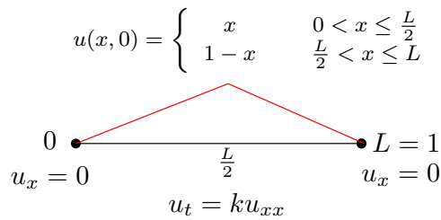
Figure 3.52: PDE specification
