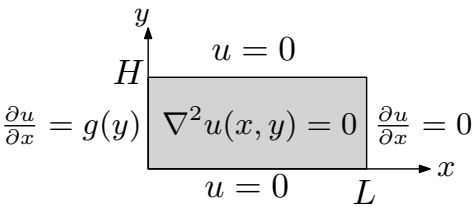
Figure 4.7: PDE specification
