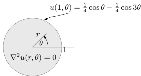
Figure 4.32: PDE specification
