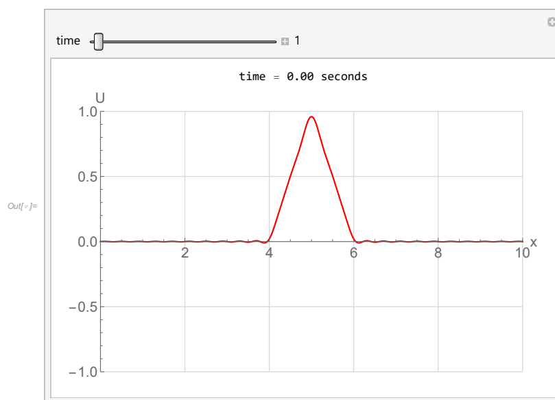
Figure 5.26: Initial state
