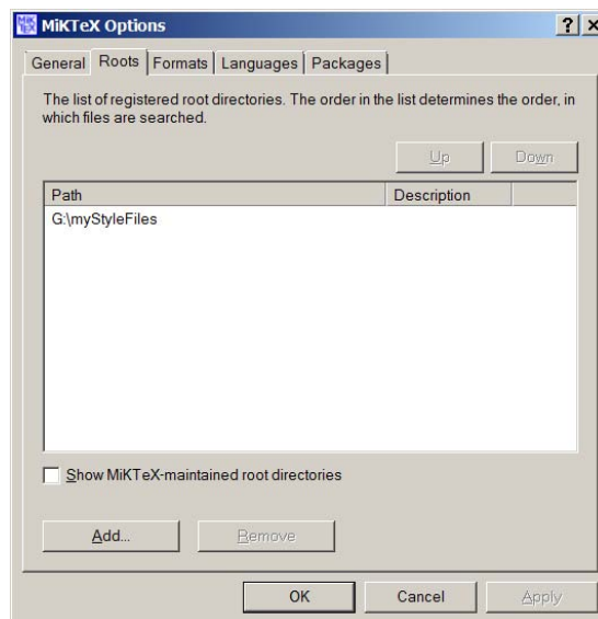
Figure 2: Selecting root
