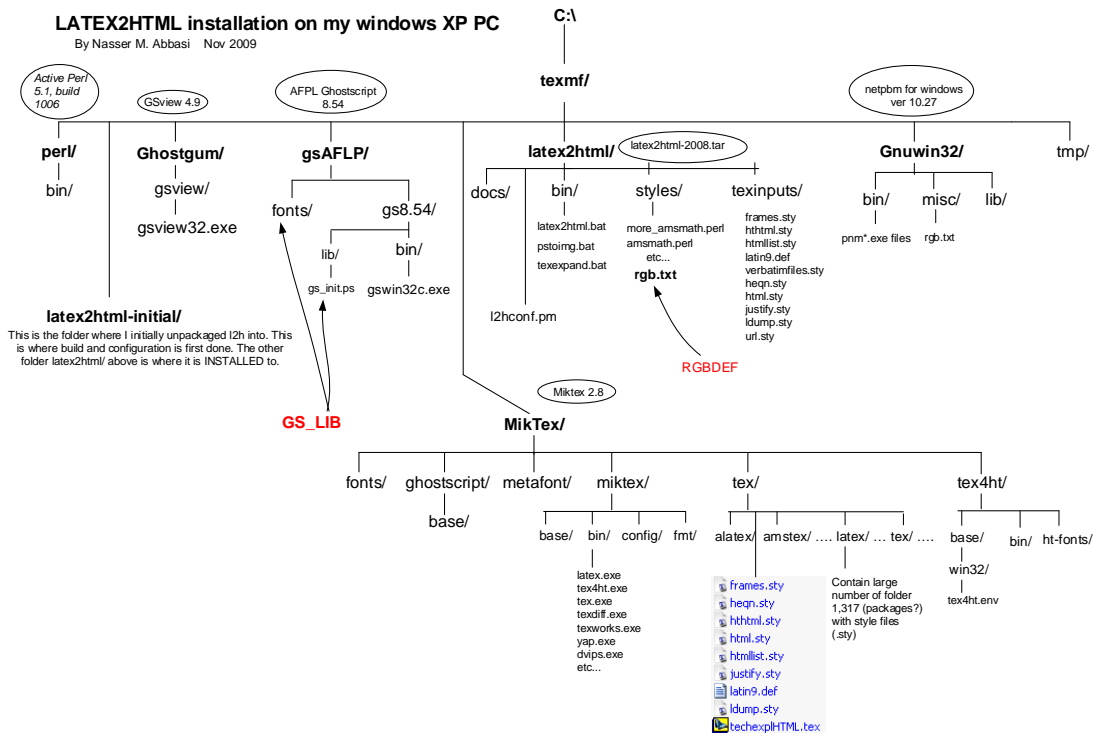
Figure 1: Installed tree
