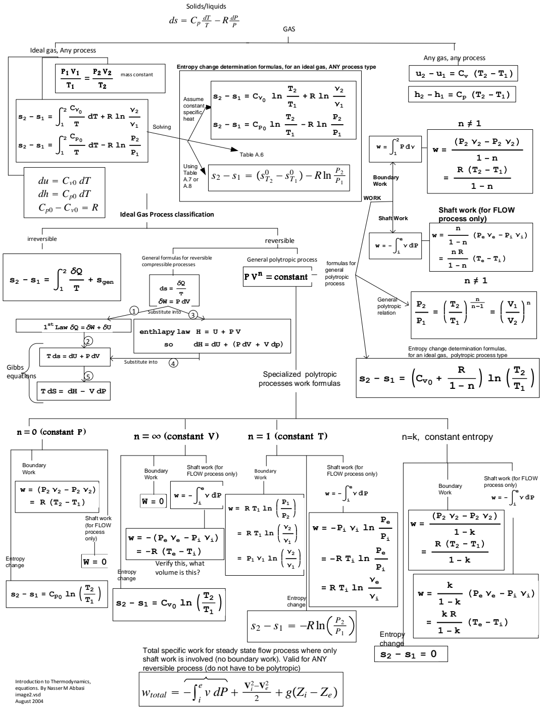
Figure 4: gas lawss
