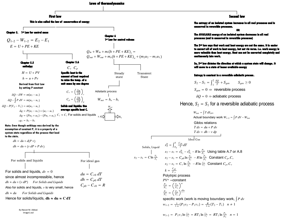
Figure 3: first and second laws diagrams
