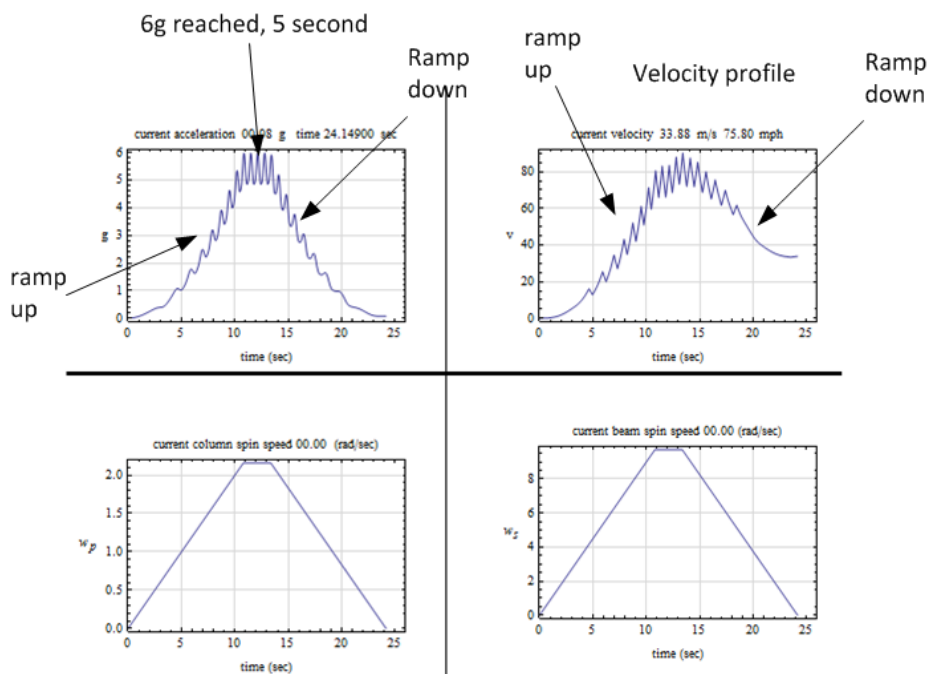
Column and beam angular velocities time histories shown effect of ramp down
