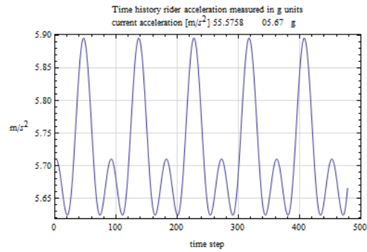
Figure 3: Time history plot for absolute acceleration of ride object for first 5 seconds
