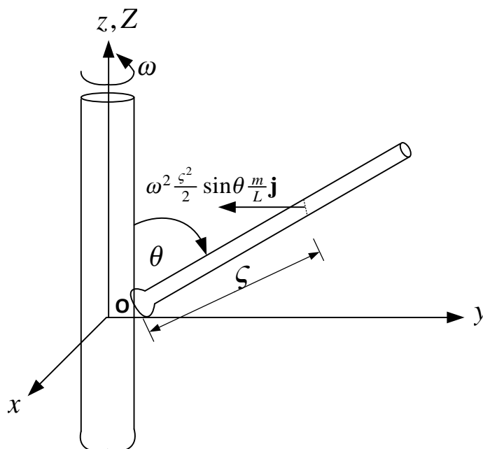
Figure 4.7: Total force acting on tube at a given distance from the shaft
