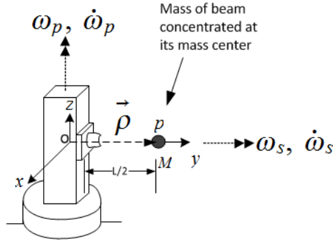
Figure 13: Rotating coordinates system xyz used to find beam center of mass acceleration
