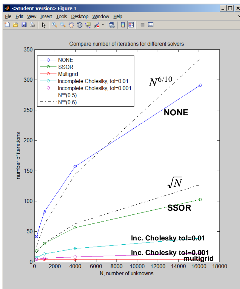
Figure 3: iterations plot
